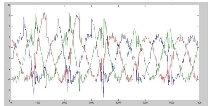
Fig.10 Source current
