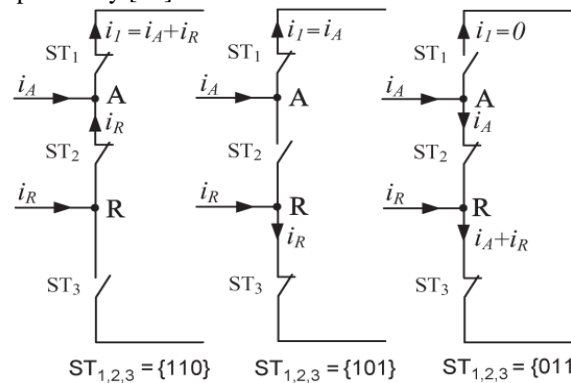
Fig.2. Three equivalent circuits for leg one of the Nine switch converter
