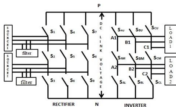
Fig. 1. Dual input Dual output indirect matrix converter
