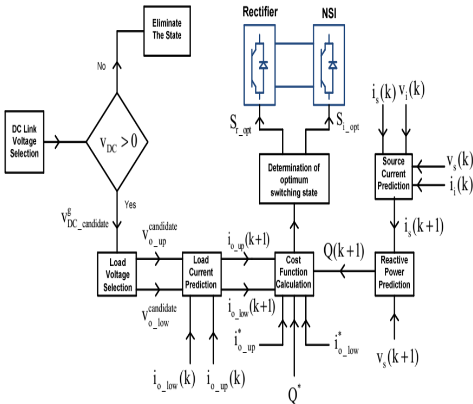
Figure 3. Model Predictive Control Scheme for Dual Output Indirect Matrix Converter
